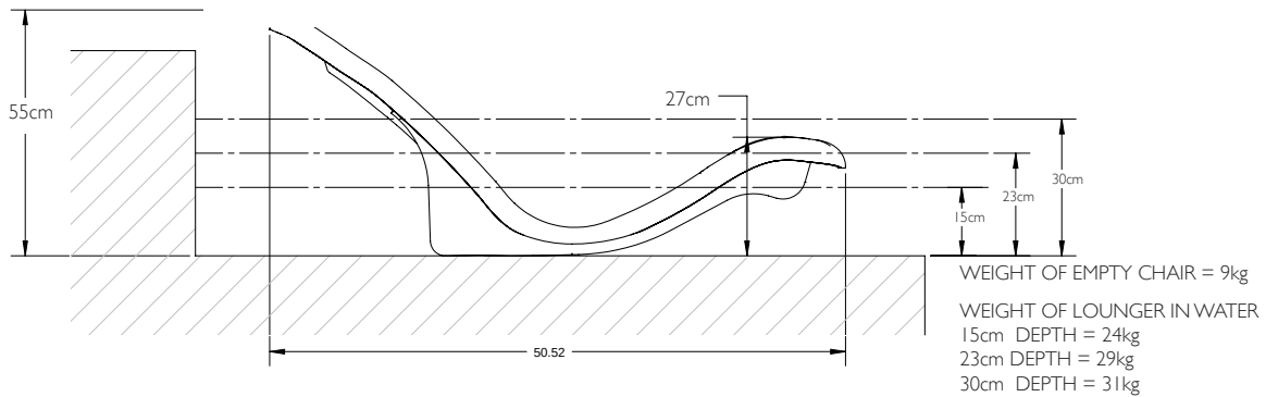
ROCKING LOUNGE CHAIR DIMENSIONS
