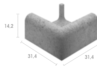
RS 938 Esquina Exterior Outside corner Angle extérieur
