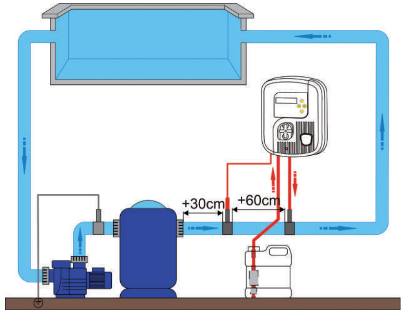
Chlor Expert MONTAJ diagram
